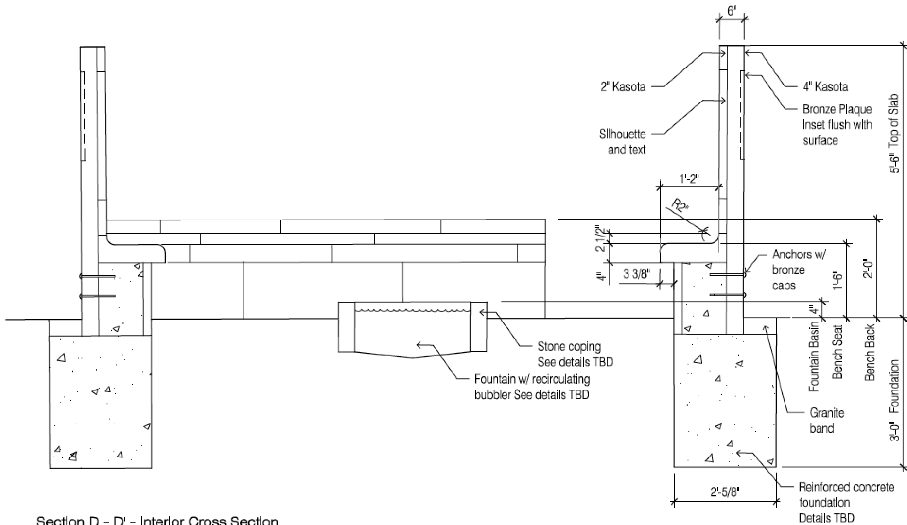
Section D - D' - Interior Cross Section
