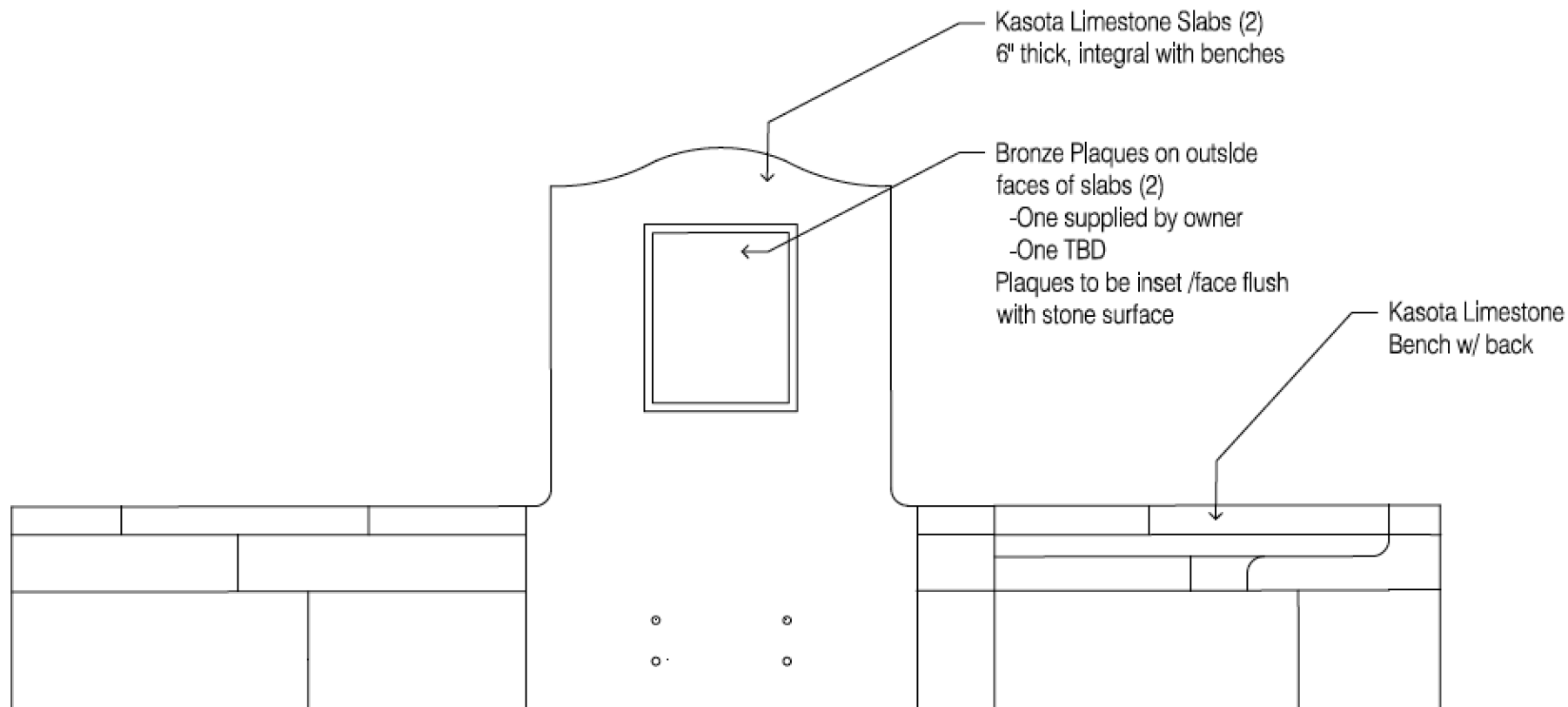
Elevation A - A' - Exterior Elevation at Entry
