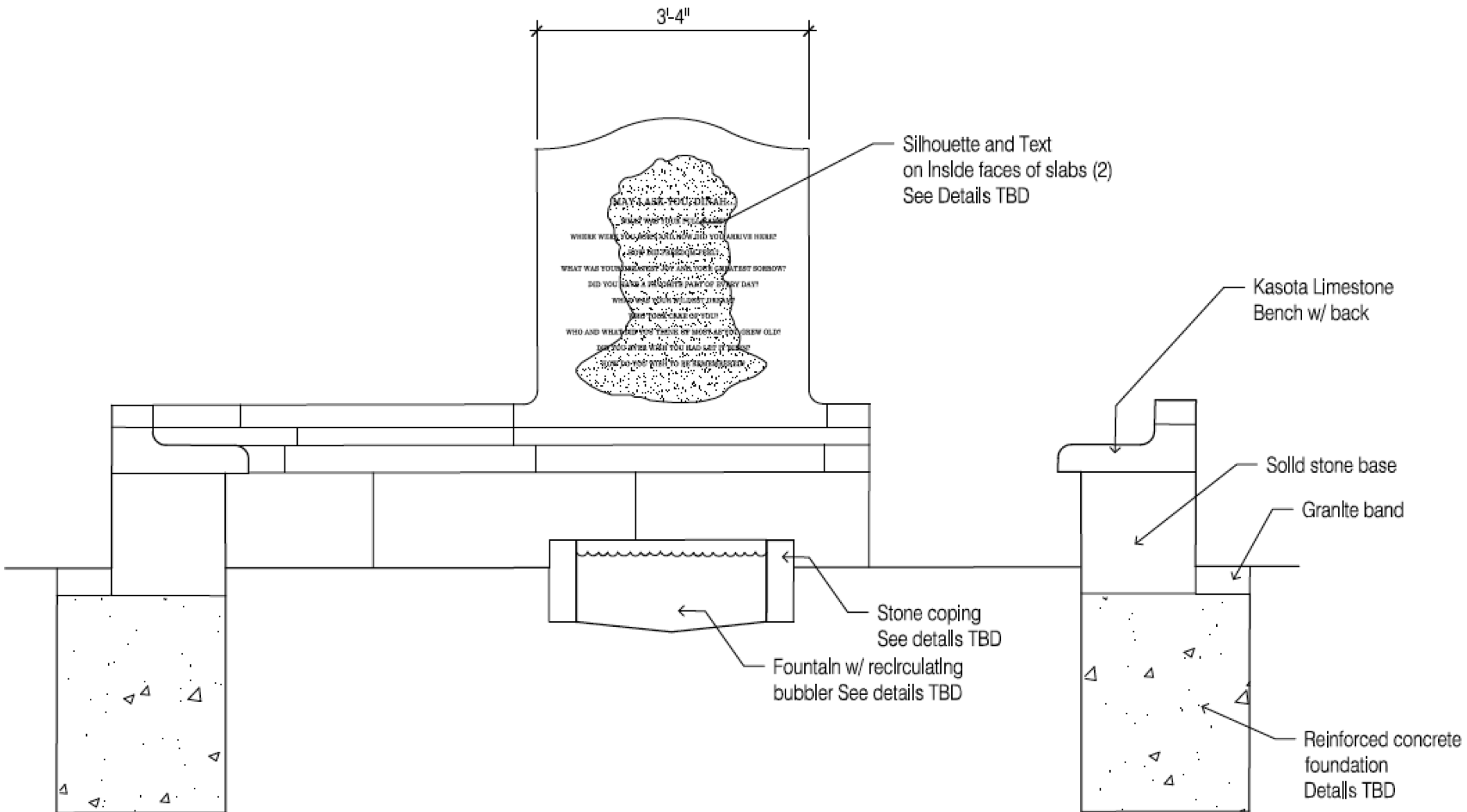
Section B - B' - Interior Cross Section Showing Slabs
